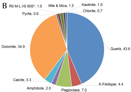
FIGURE 4 X-ray diffraction analysis of sand mineralogy. a) High percentage of hard silica minerals such as quartz, feldspar (including plagioclase), amphibole, and phyllosilicates (clay) creates durable sand. b) Less durable sand is formed by grains with a high proportion of soft carbonate minerals such as calcite and dolomite.
